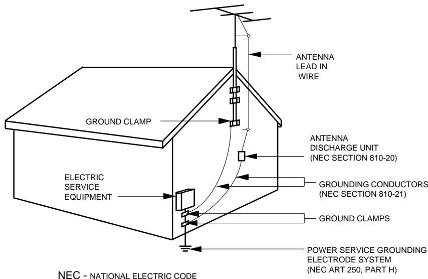
EXAMPLE OF ANTENNA GROUNDING
