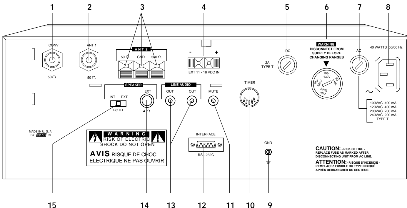
FIGURE 6 REAR PANEL
