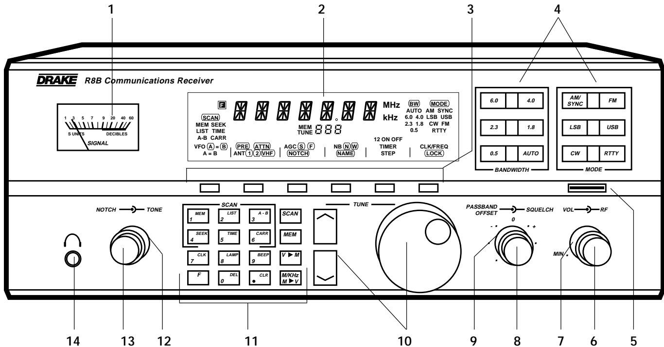
FIGURE 4 FRONT PANEL
