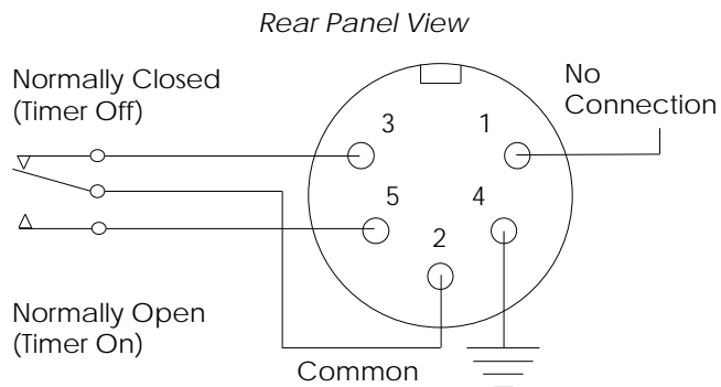
Figure 15 Timer Connections Contacts shown with TIMER OFF
