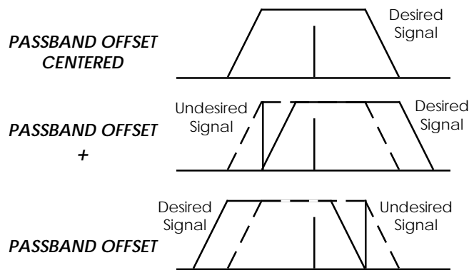
FIGURE 9 PASSBAND OFFSET Operation
